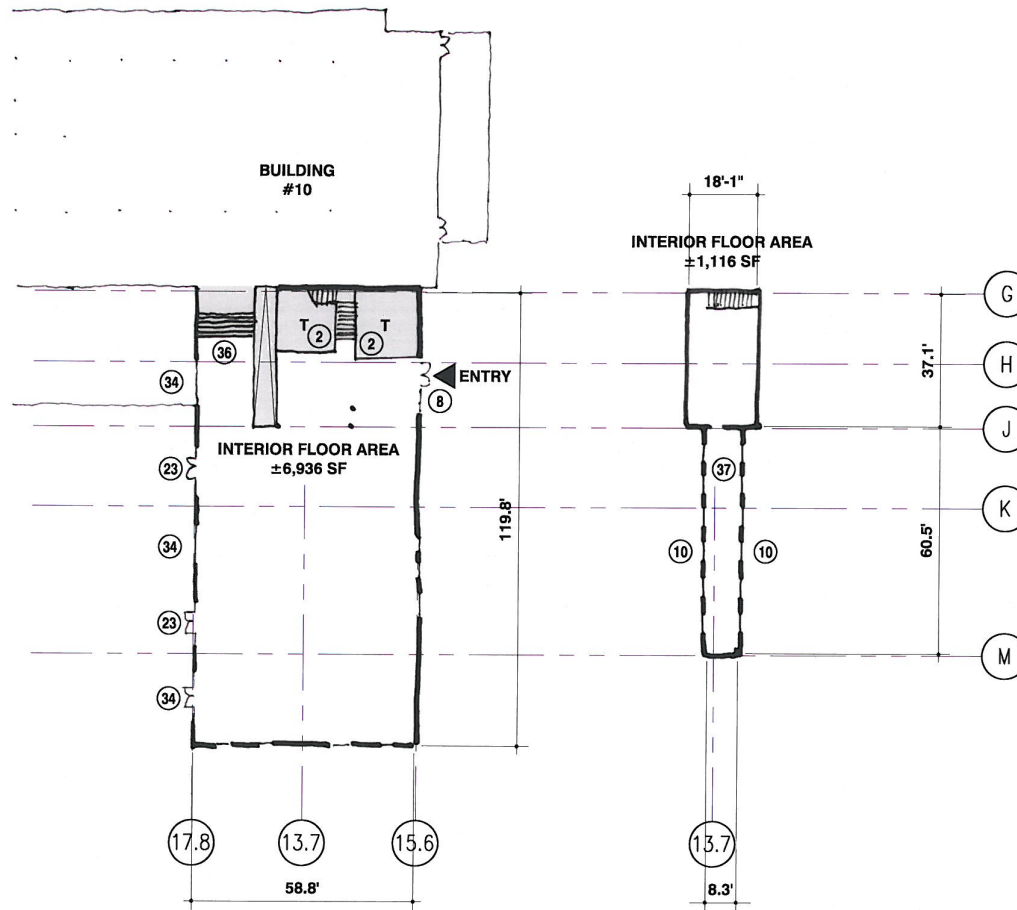
SECOND FLOOR PLAN SCALE: 1/32"=1'-0"
